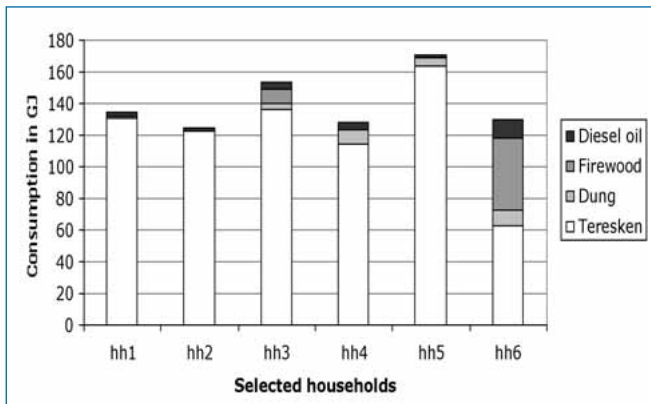
Figure 2.29: Annual Energy Consumption at the Household Level. Annual energy consumption in GJ of six selected households in Nisur. Source: Field study 2003
