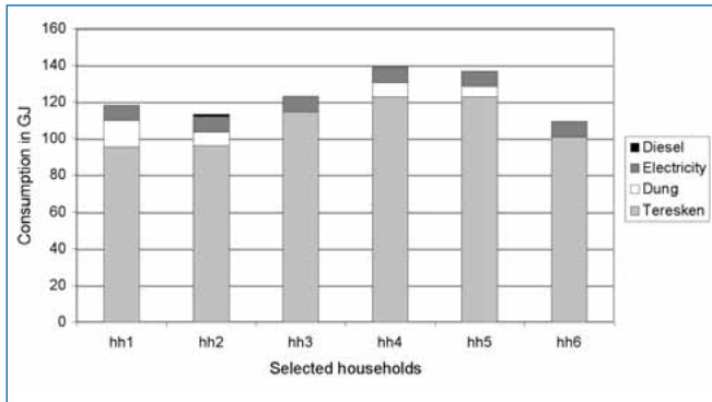
Figure 2.22: Annual Energy Consumption in GJ of Six Selected Households in Savnob. As mentioned in the MHPS section of this chapter, there is no data available concerning a household's individual electricity consumption, thus in this diagram all customers use the same amount of electricity. Source: Field study 2003
