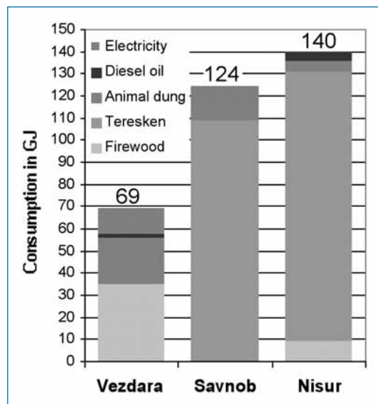
Figure 2.35: Overall Annual Energy Consumption in GJ per Household. Comparison of the three case study villages regarding annual mean household energy consumption.
